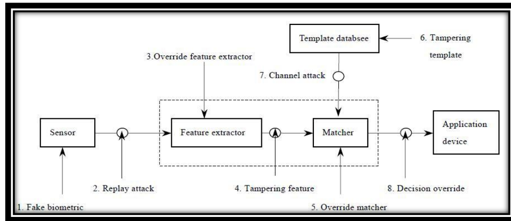
Fig 4 attack point on biometric system
